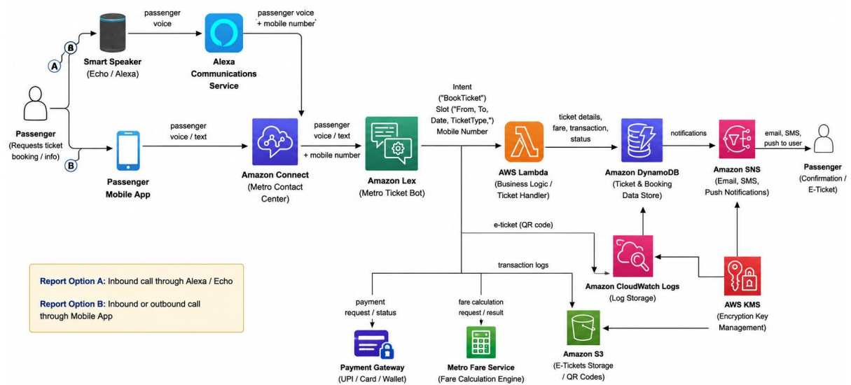
Metro Ticket Generating System – High Level Architecture
